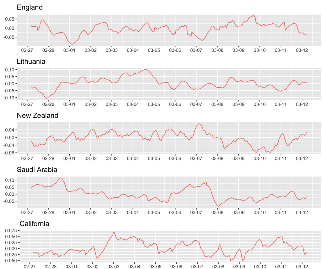
Fig. 1. Normalized average IBI with 24-hour moving average smoothing.
